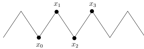
Figure 1. The zig-zag graph.
