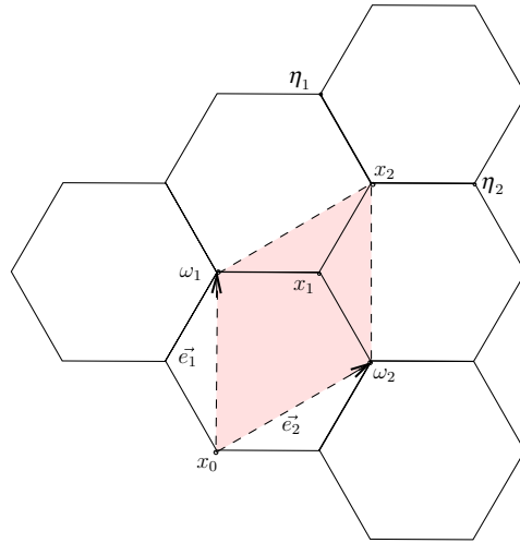
Figure 2. The honeycomb graph. (This figure is in colour only in the electronic version)
